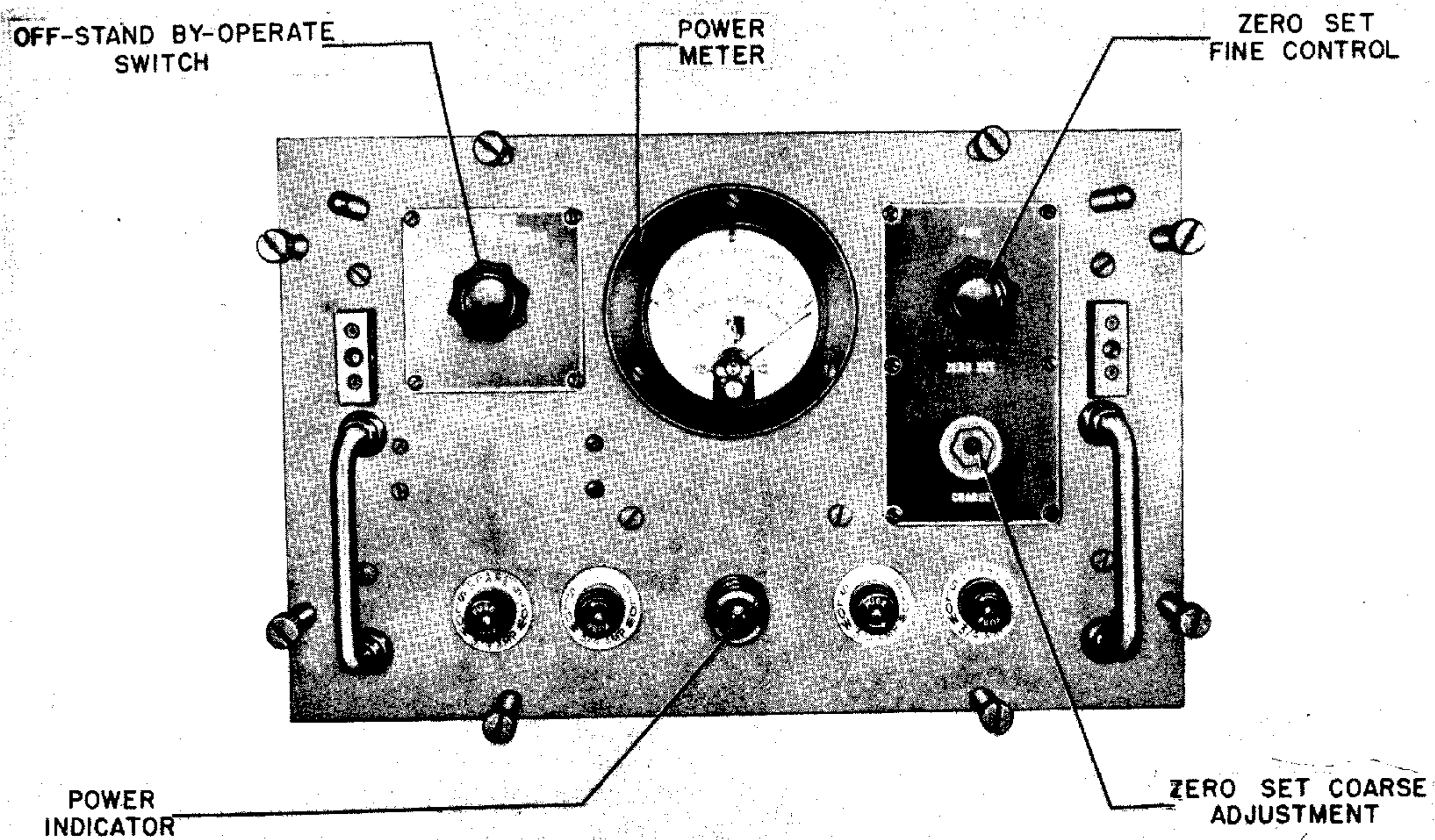
Figure 3-4. Power Monitor, Control Panel
