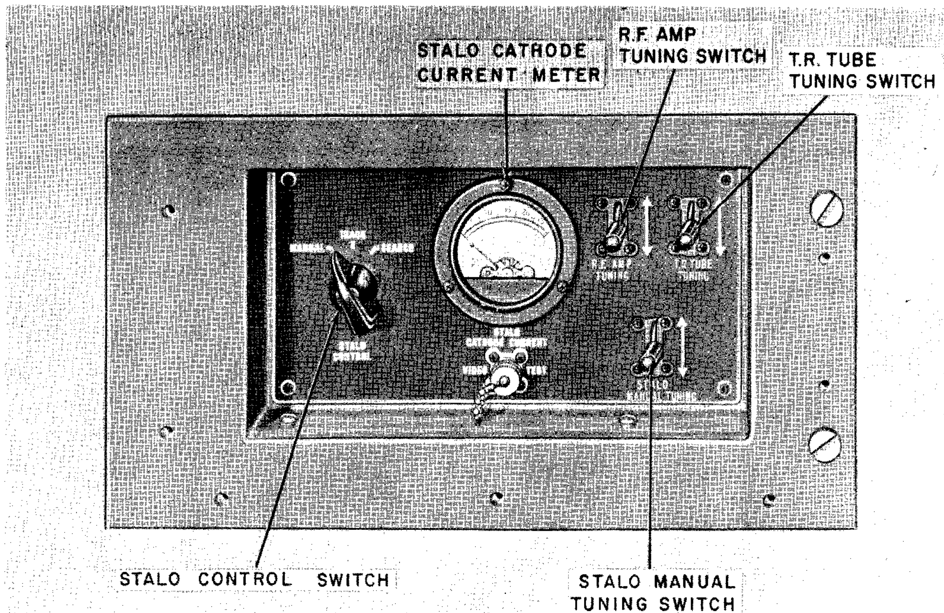
Figure 2-9. Receiver RF Group, Lower Control Panel
