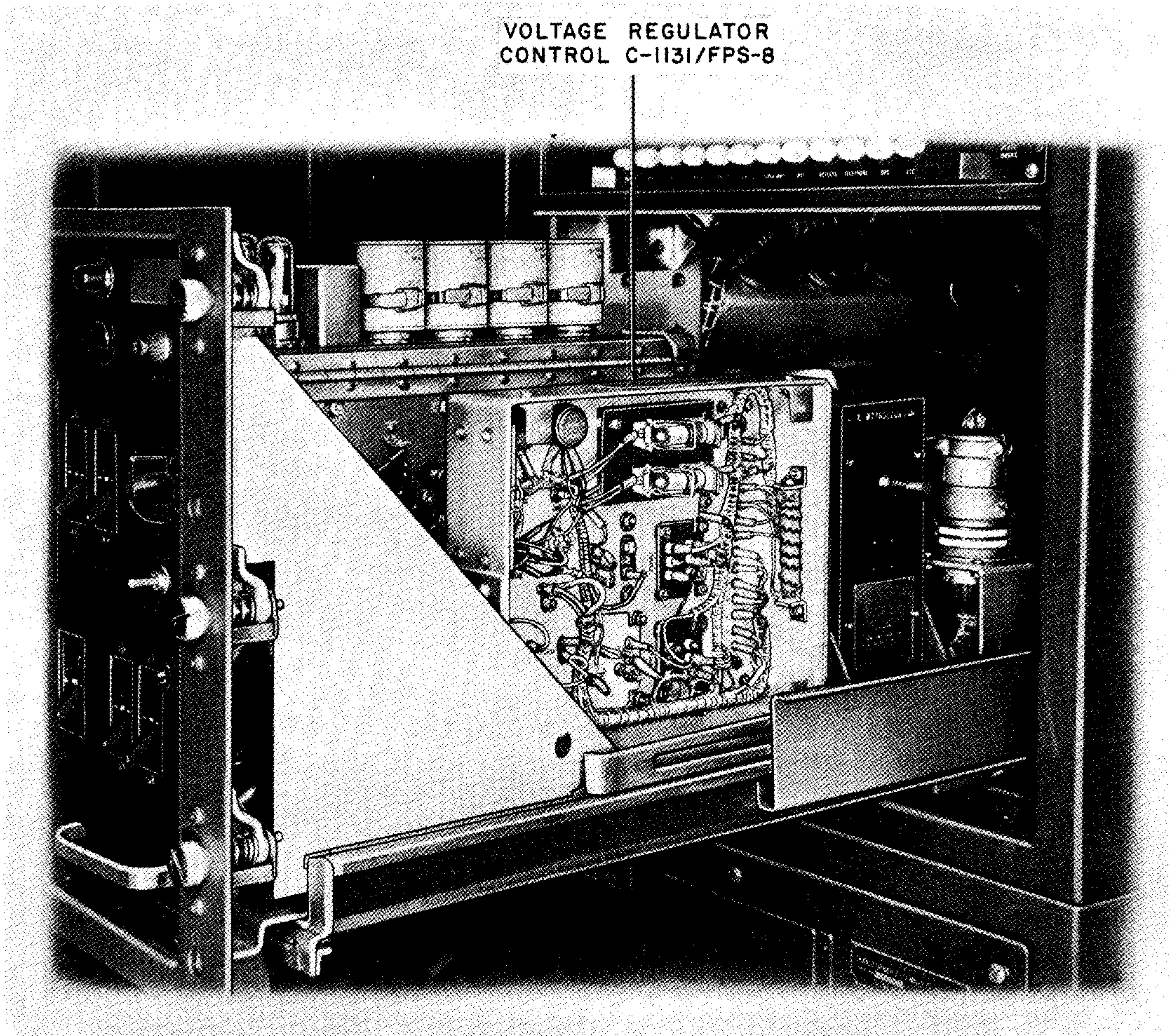
Figure 1-35. Power Distribution Unit, Right Side of Extended Drawer, with Cover Plate Removed
