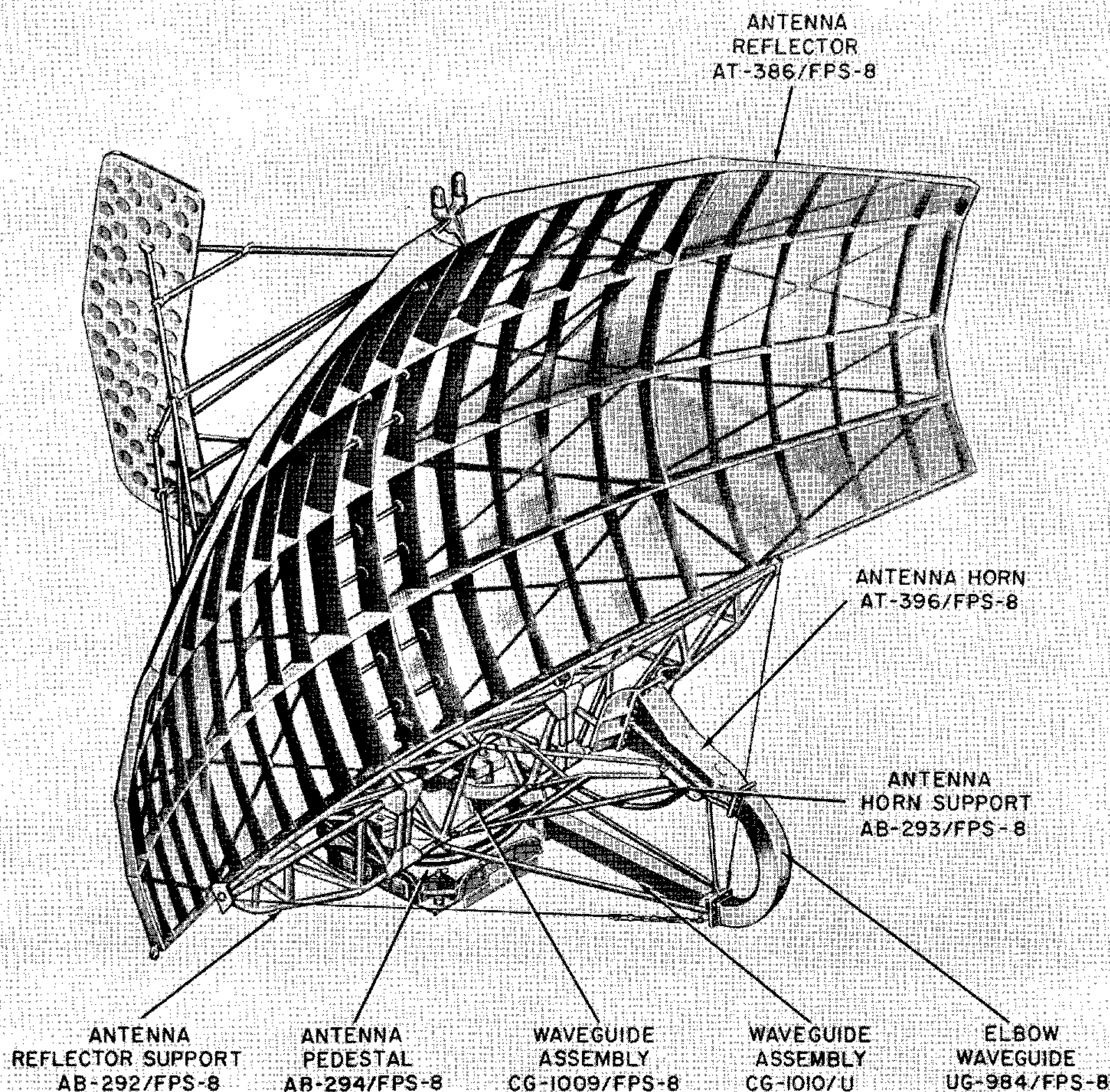
Figure 1-12. Antenna Group OA-405/FPS-8
