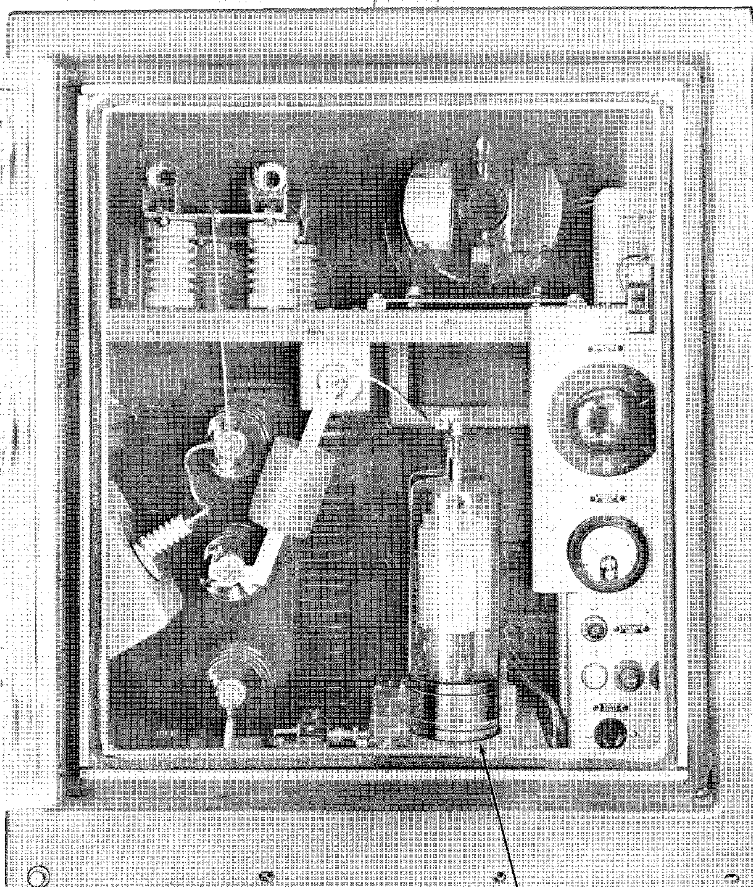
MODULATOR SUBASSEMBLY MX-1962/FPS-8
