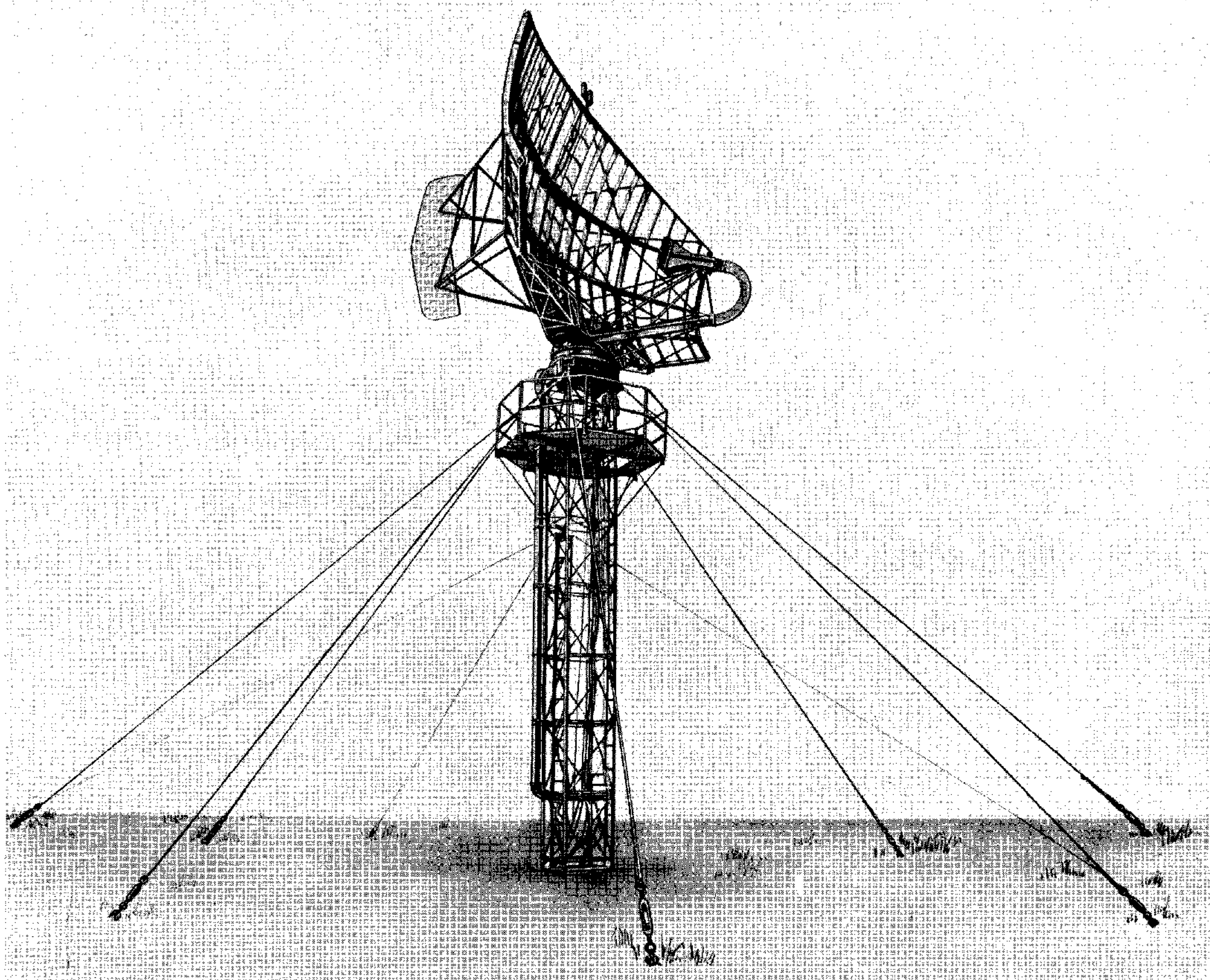
Figure 1-5. Tower AB-396/MPS
