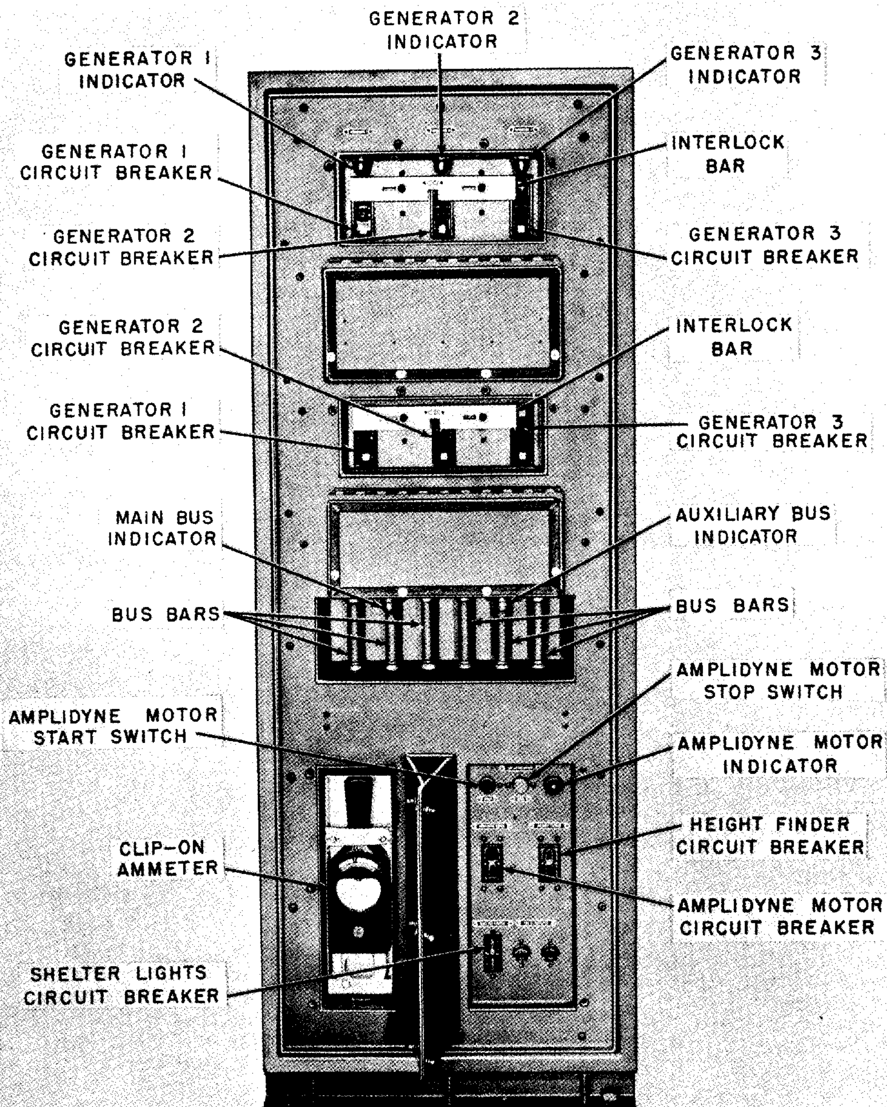
Figure 2-1. Power Control Box, Front Panel
