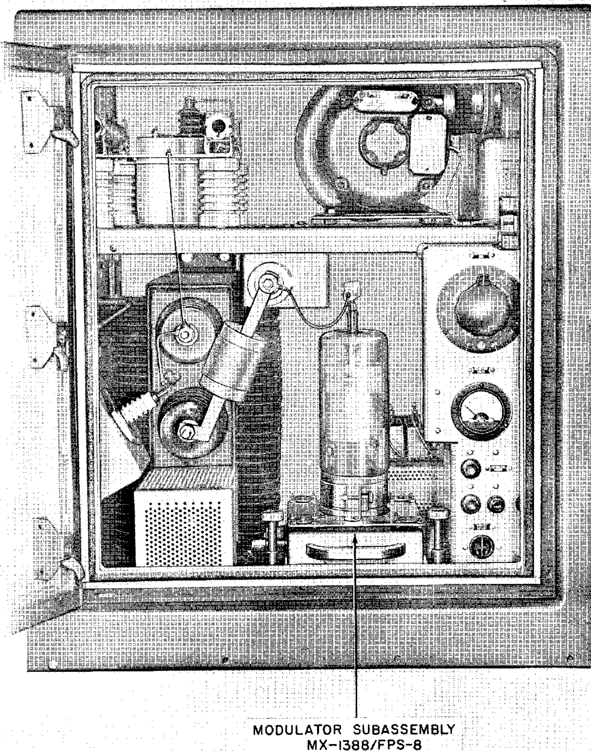
Figure 1-9. Modulator Group OA-414/FPS-8, Upper Section, Interior View
