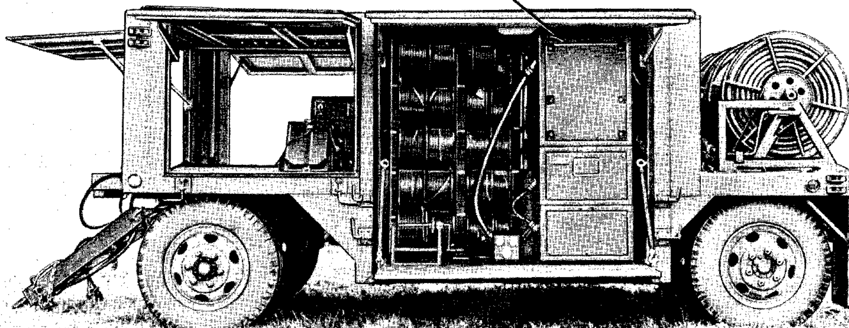
Figure 1-4. Trailer, Van V-113/MP5-11
