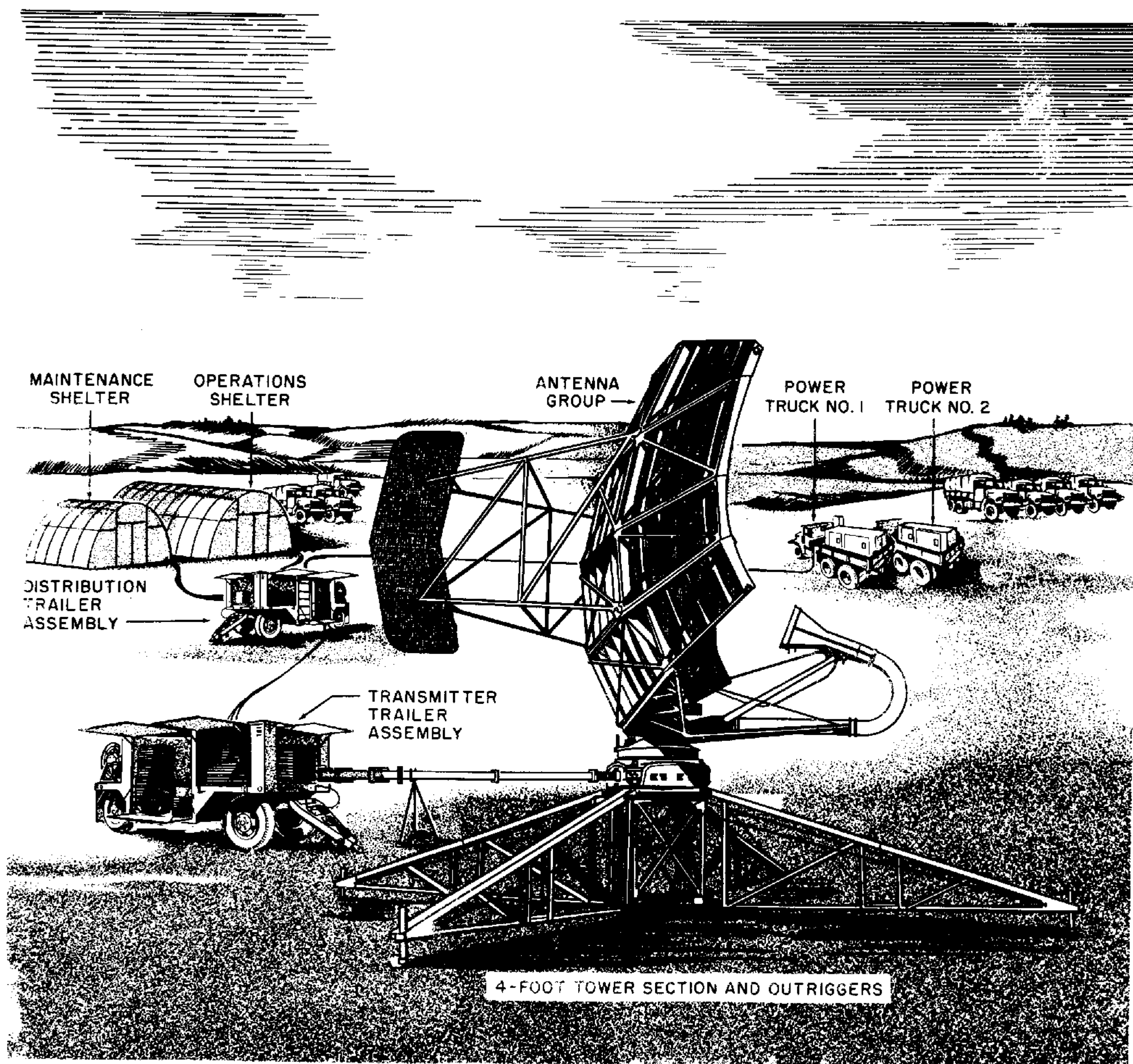
Figure 1-2. Radar Set AN/MPS-11
